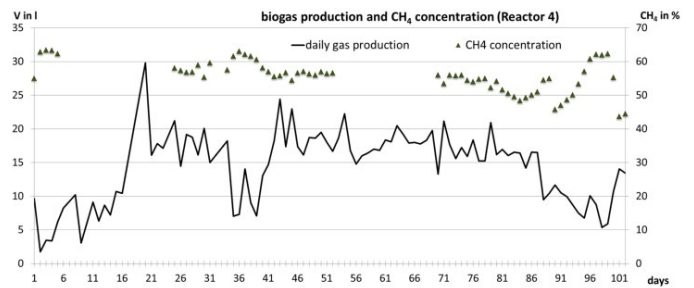
Figure 9. Biogas production and CH 4 concentration, semi continuous exp. of 50% rachis, 50% banana.
