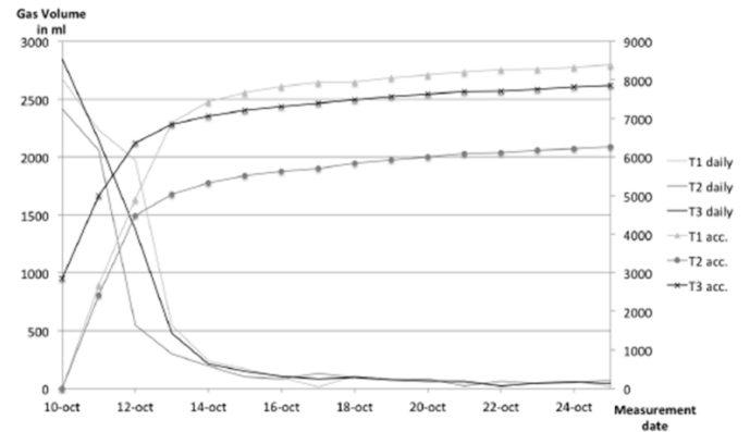
Figure 4. Biogas production from whey in the batch system.
