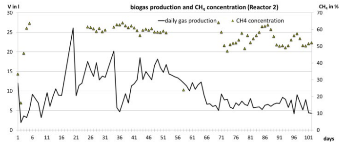
Figure 7. Biogas production and CH 4 concentration, semi continuous exp. of 66 % rachis, 33 % banana.
